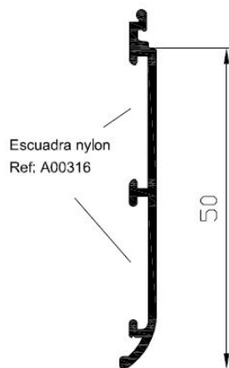
Solape 50 mm Ref: 4150
