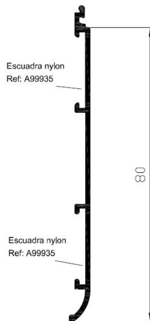
Solape 80 mm Ref: 4180
