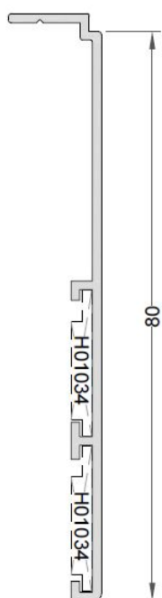
Solape compacto 70 Ref: 8480
