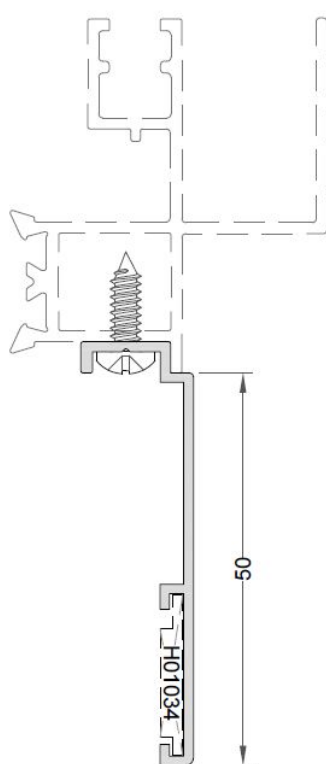
Solape resalte 50 Ref: 9450
