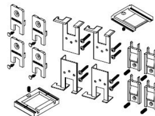
Kit CONFORT-80 Ref.: H19016
