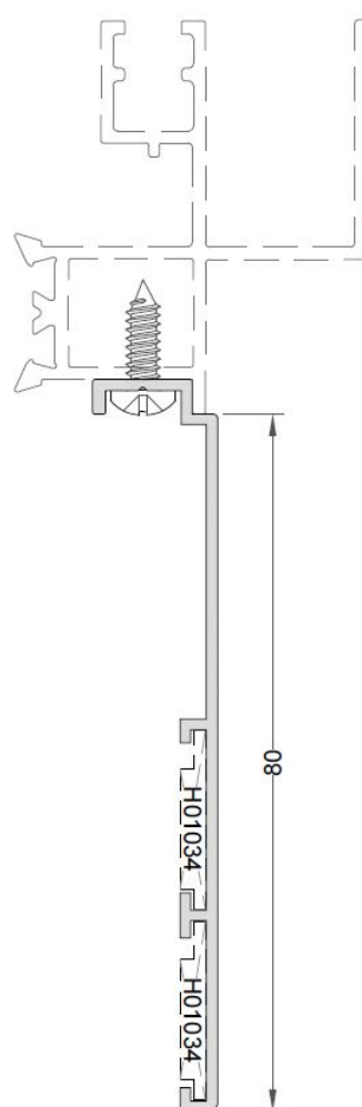
Solape resalte 80 Ref: 9480
